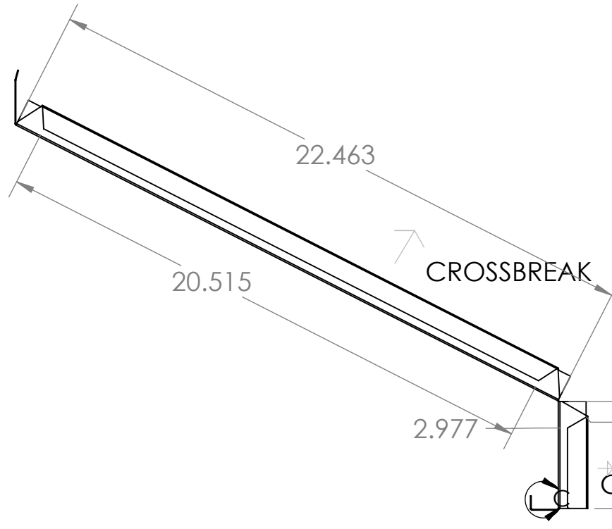
DETAIL J SCALE 2 : 1
